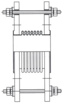
PLAN VIEW OF A TYPICAL APPLICATION EXAMPLE
